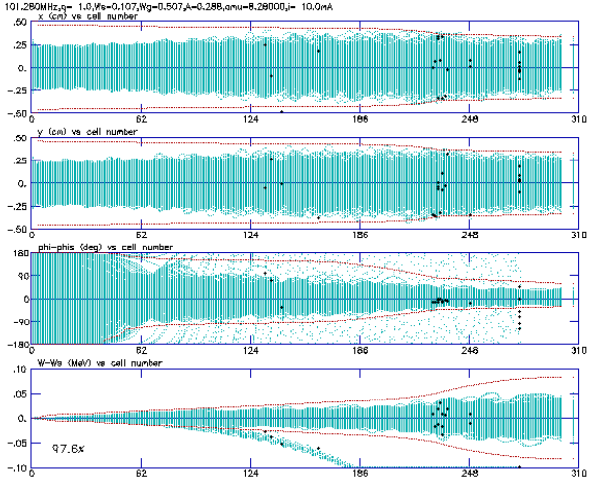
Figure 2: Evolution of beam parameters versus cell number as simulated with PARMTEQM. The dashed line indicates the physical aperture.
