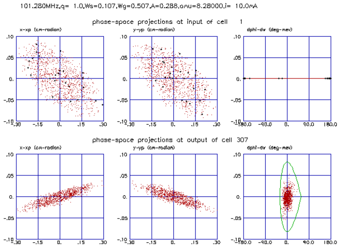
Figure 1: Input (upper plots) and output (lower plots) beam of the RFQ as simulated with PARMTEQM.
